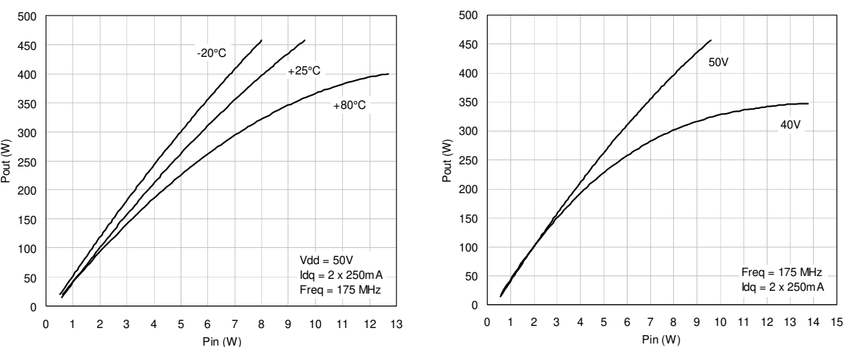
Figure 8. Pout Vs Input Power and Case Temp Figure 9. Pout Vs Input Power & Drain Voltage
