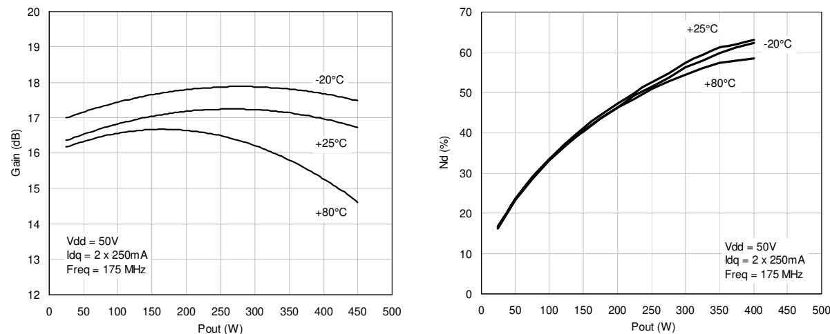
Figure 6. Power Gain Vs Pout and Case Temp. Figure 7. Efficiency Vs Pout and Case Temp.
