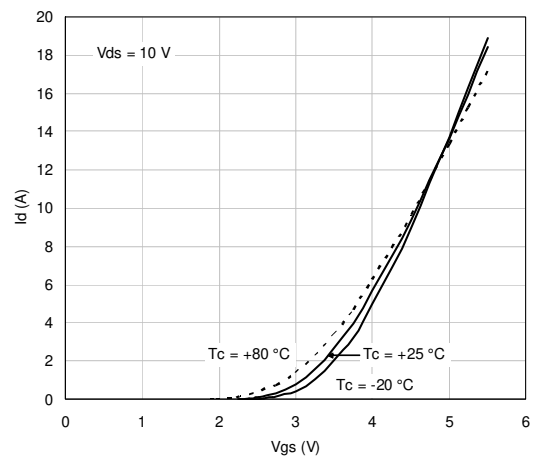
Figure 3. Drain Current Vs Gate Voltage
