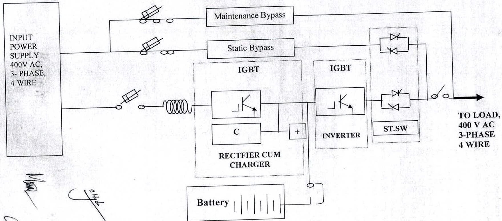
FIGURE -1 UPS SINGLE MODULE -SUGGESTIVE CONFIGURATION
