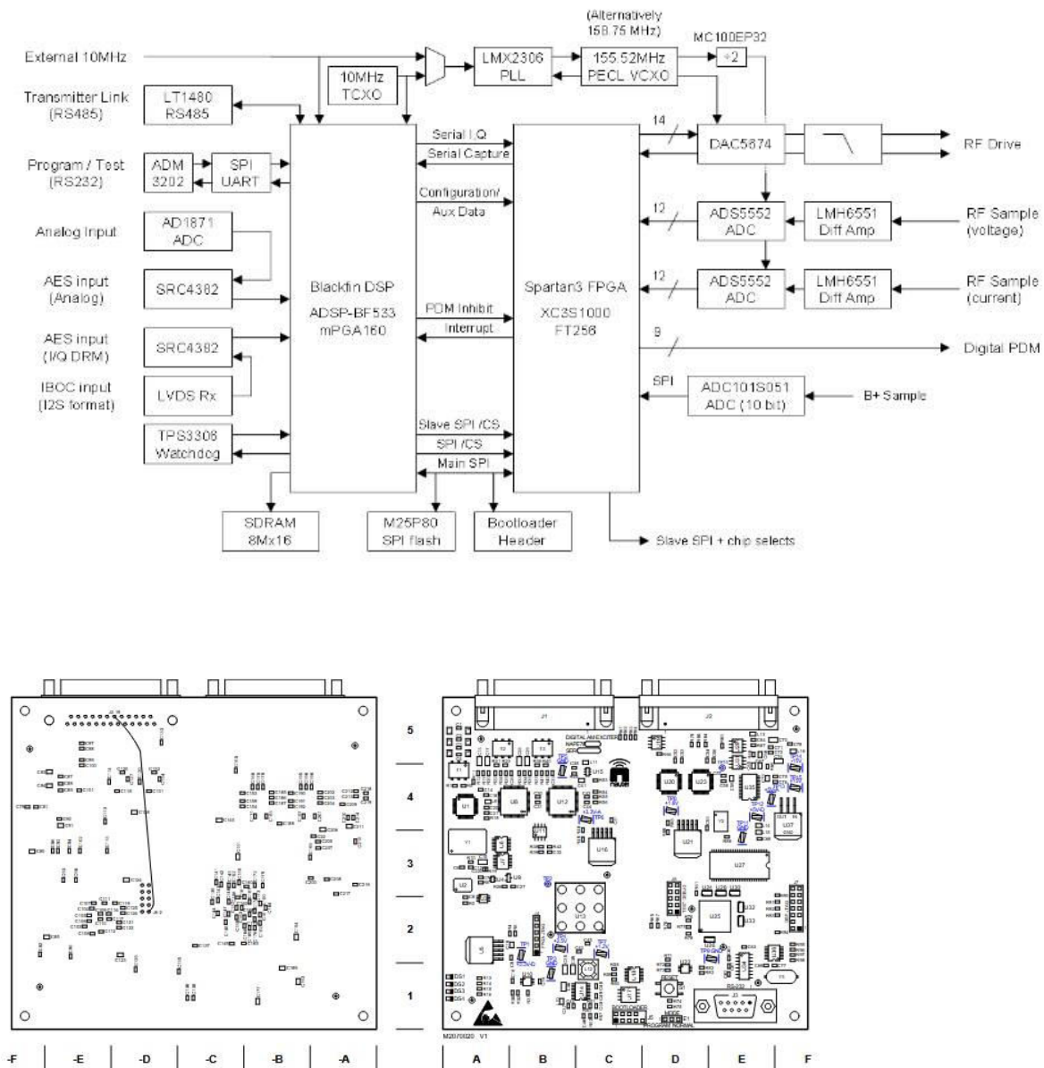
Figure 2.1: Block Diagram - Digital Exciter Block Diagram
